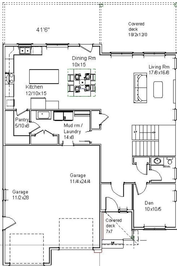
1st FLOOR PLAN 1300sqft
